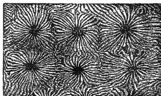
SMITHIA PENGELLYI. ( Old Red Sandstone. )
